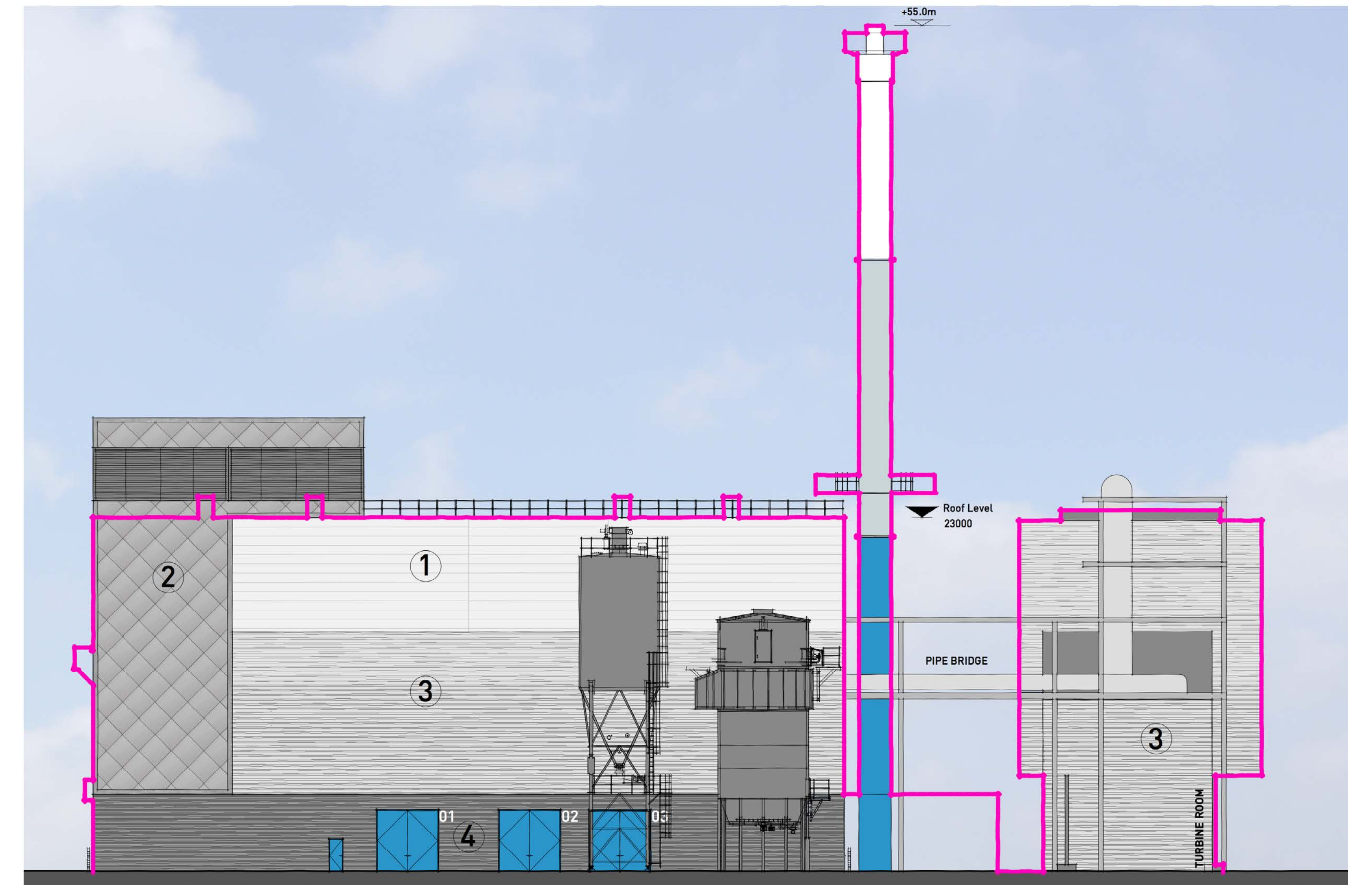
SOUTH ELEVATION
