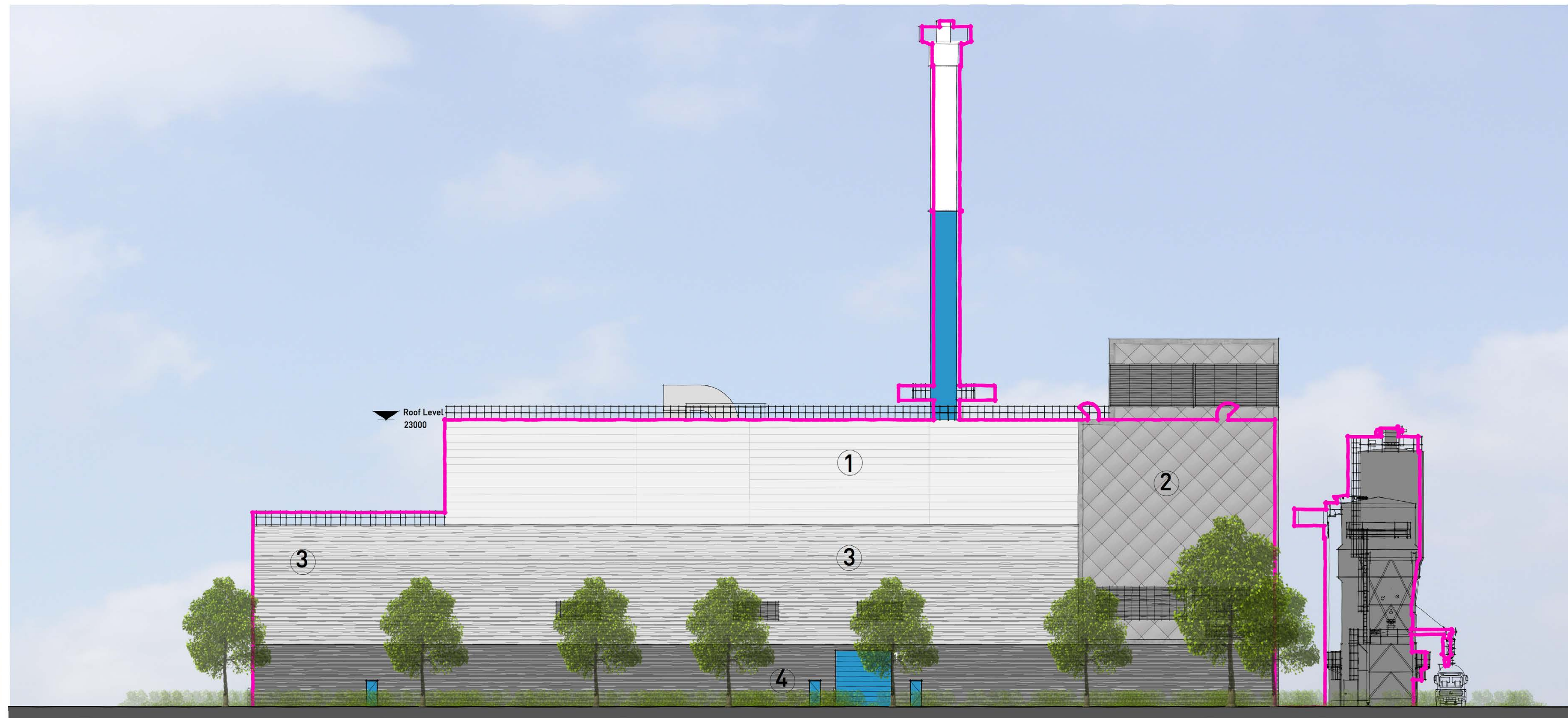
WEST ELEVATION
