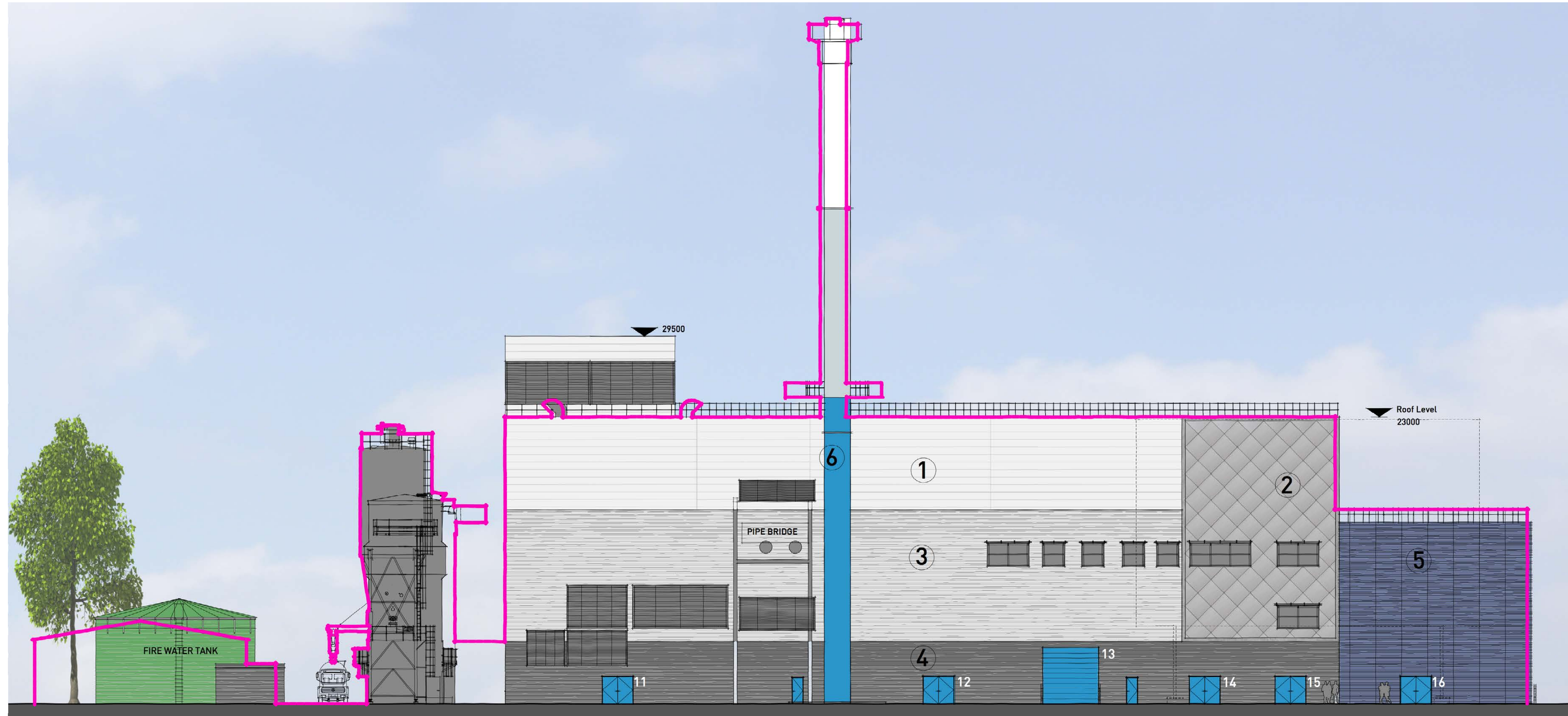
EAST ELEVATION
