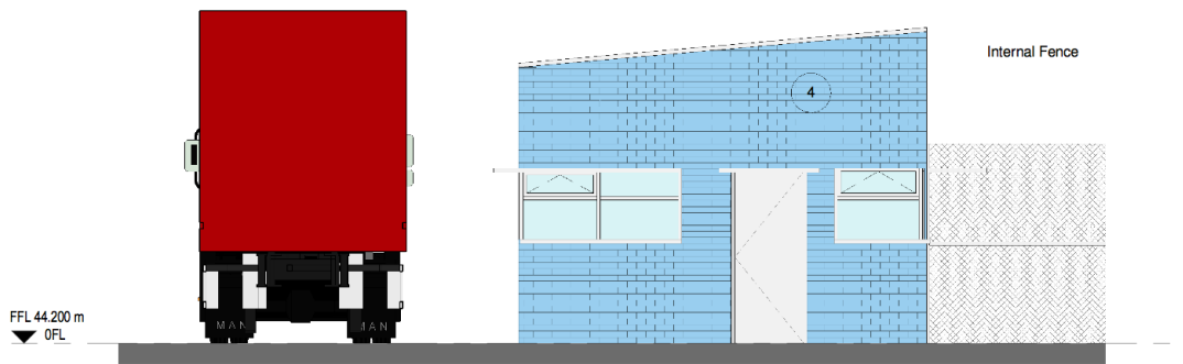
4 Gatehouse South elevation
