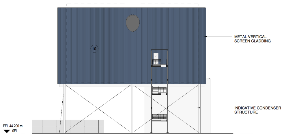
3 ACC Building South Elevation
