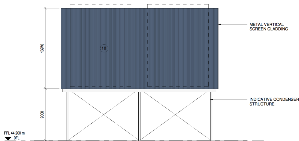
2 ACC Building North Elevation
