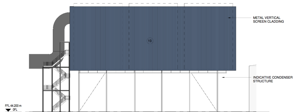
4 ACC Building East Elevation
