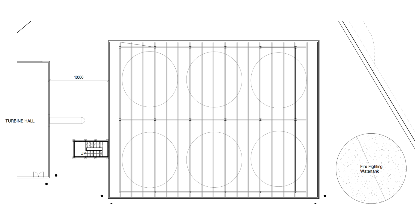
1 ACC Plan
