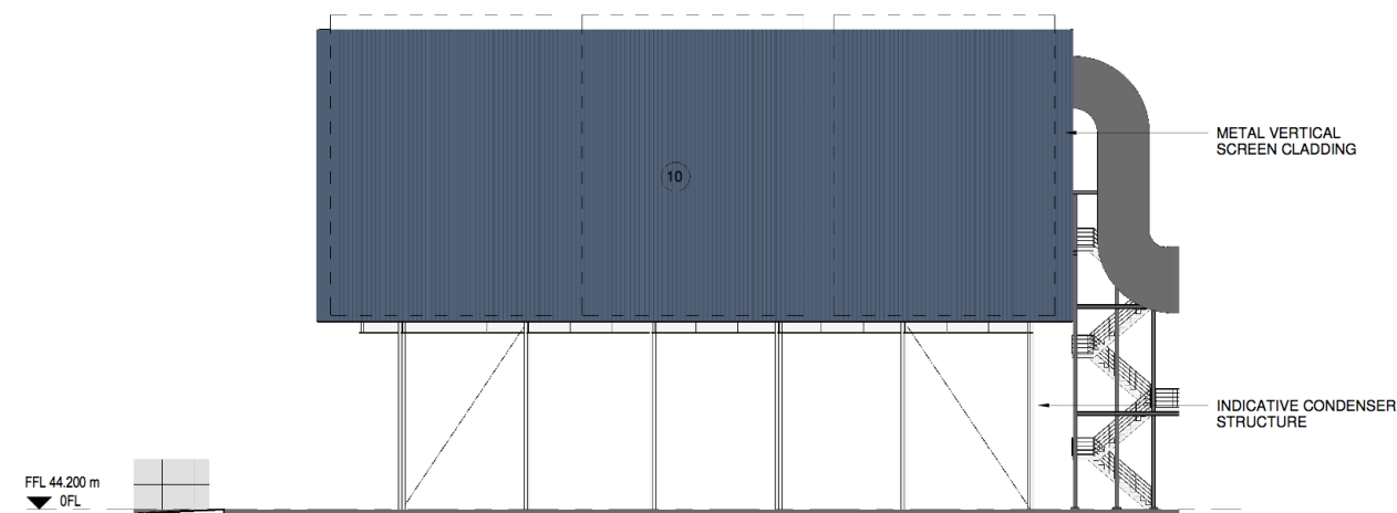
5 ACC Building West Elevation
